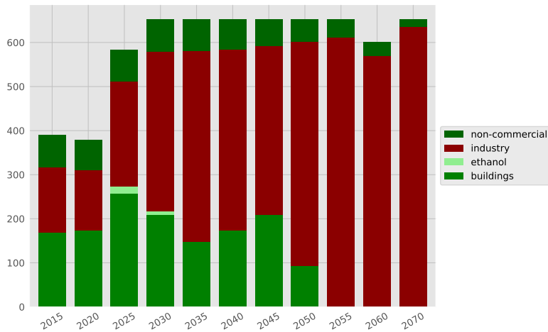
Biomass utilization (PJ)
